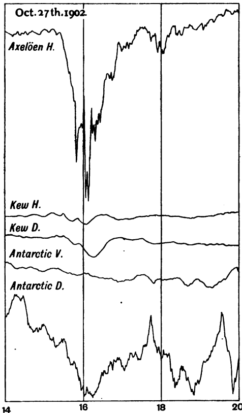
FIG. 27.—ARCTIC-KEW-ANTARCTIC CURVES.
